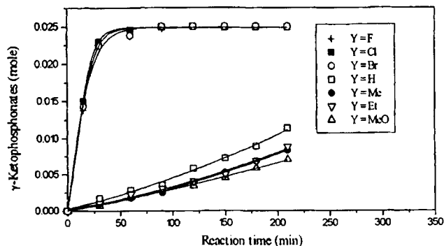
FIGURE 1 The effect of substituents on the formation of aryl \gamma -ketophosphonates 3 with the same initial mole of \beta -chloroethyl aryl ketones 1 in 0.025 mole
