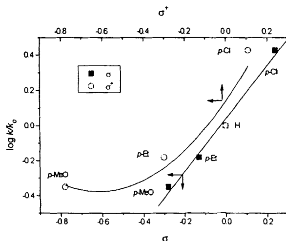
FIGURE 2 Hammett plot of phosphonation of substituted aryl ketones 1 with TEP using \sigma and \sigma^+
