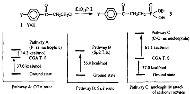
FIGURE 3 Energy requirements for different reaction pathways (Y=H) by AM1 calculation
