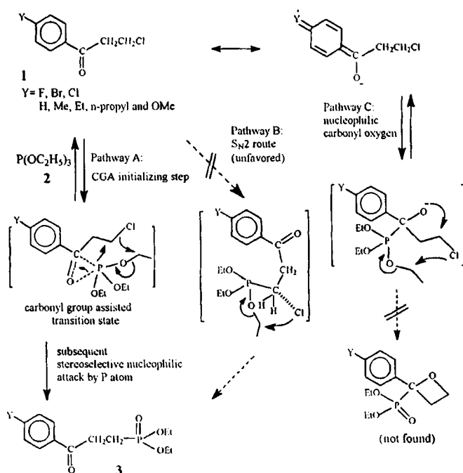
SCHEME 1 Multi-stereoselective pathways for phosphonation of \beta -chloroethyl aryl ketones 1
